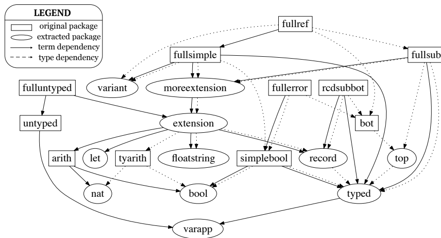
■ Figure 12 Package dependency graph.
